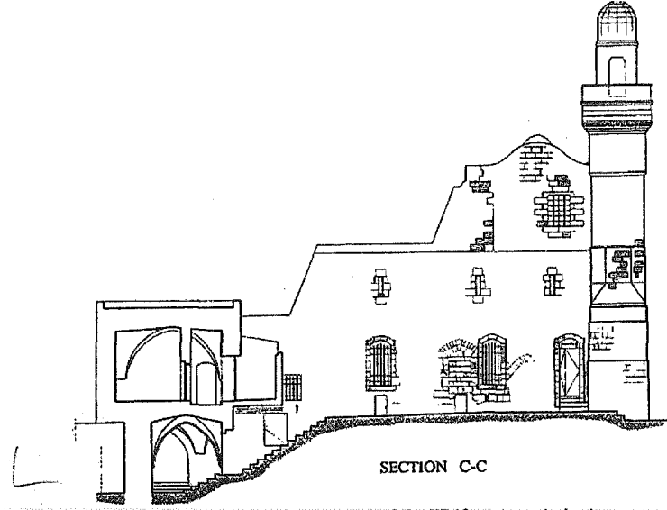
Fig. 19.5 Al-Khanqah al-Maulawiyya, sections B-B and C-C (courtesy of the Welfare Association).
