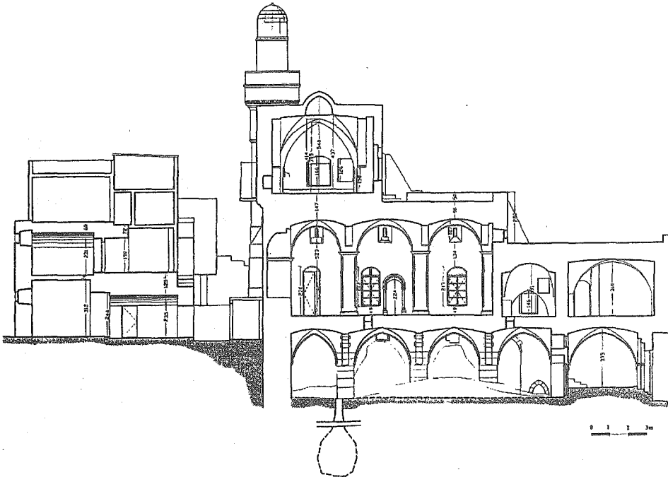
Fig. 19.6 Al-Khanqah al-Maulawiyya, section A-A (courtesy of the Welfare Association).
